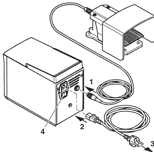
连接方法见上图 See above diagram for the connection.
