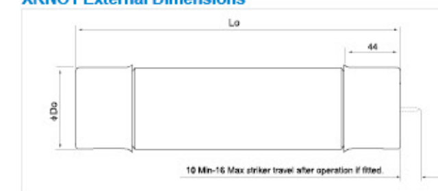
XRNO1 External Dimensions
