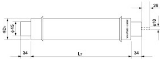
XRNT □ Fuse link
