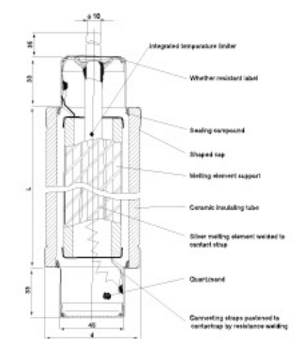
RN Series H.V. Fuse Link Cross Section
