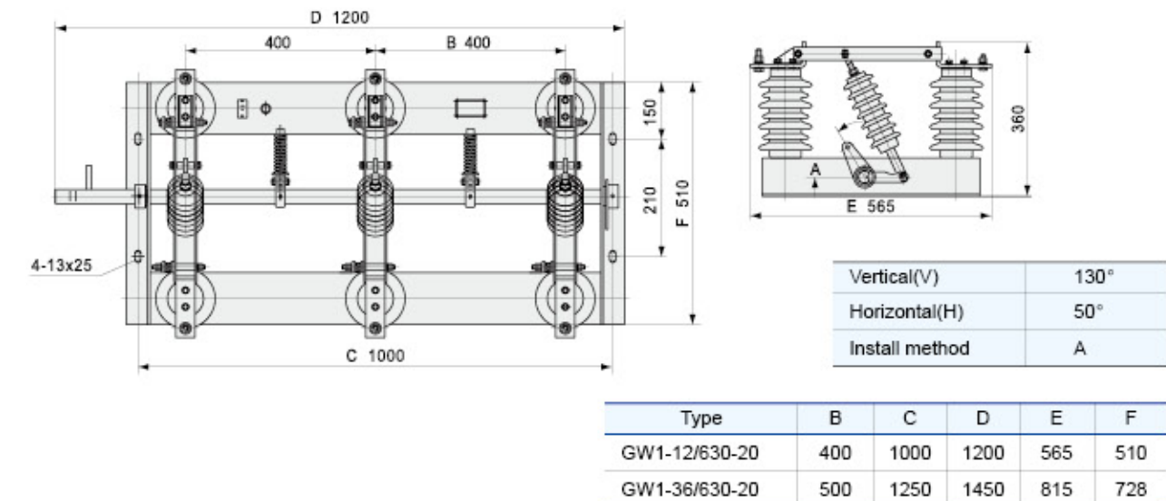
Fig.2 GW1-12, 36D with earthing blade
