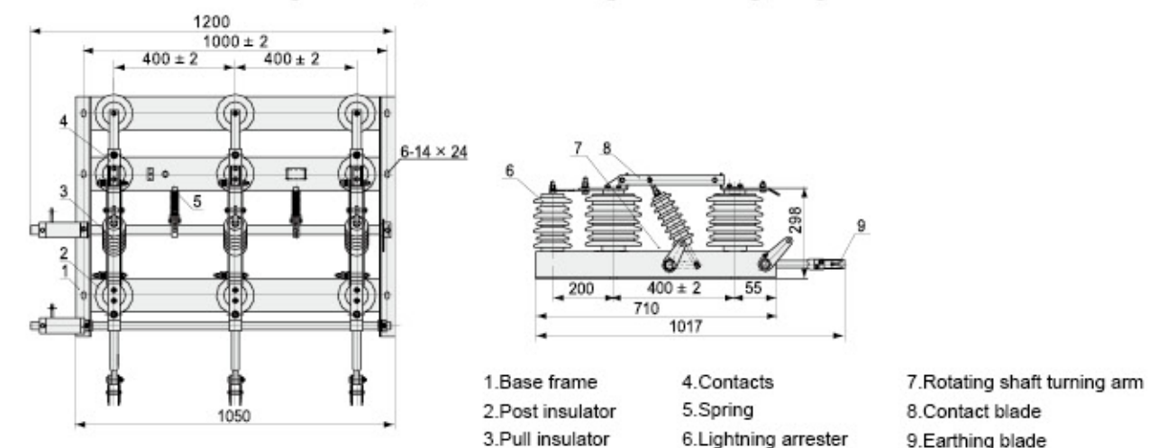
Fig.3 GW1-12, 36D with earthing blade and lightning arrester
