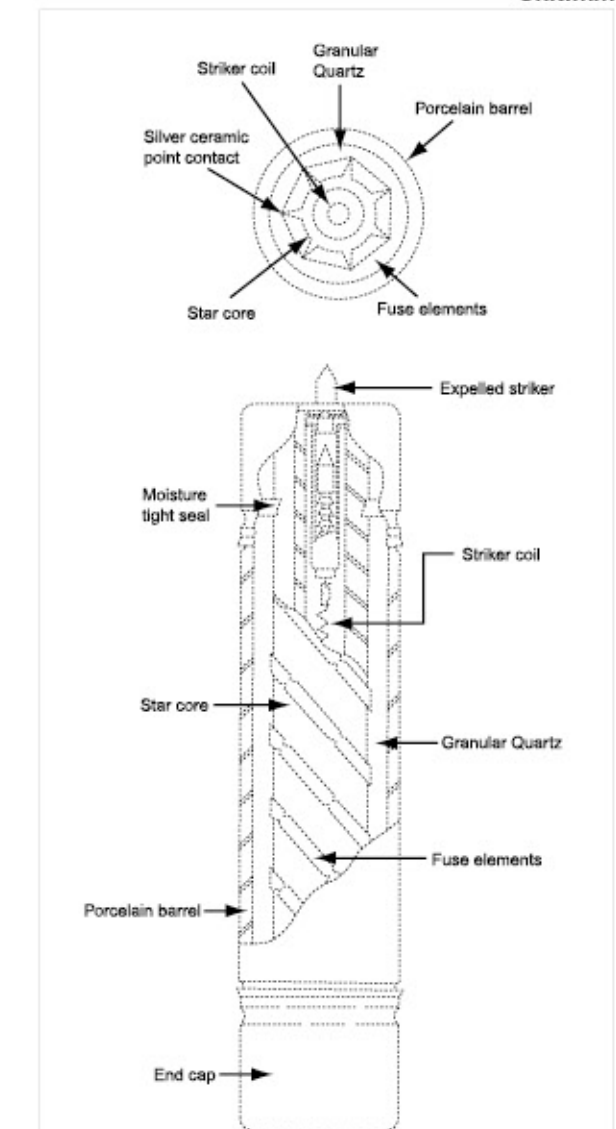
BS&DIN Type H.V. Fuse Link Cross Section Compared Unit:mm
